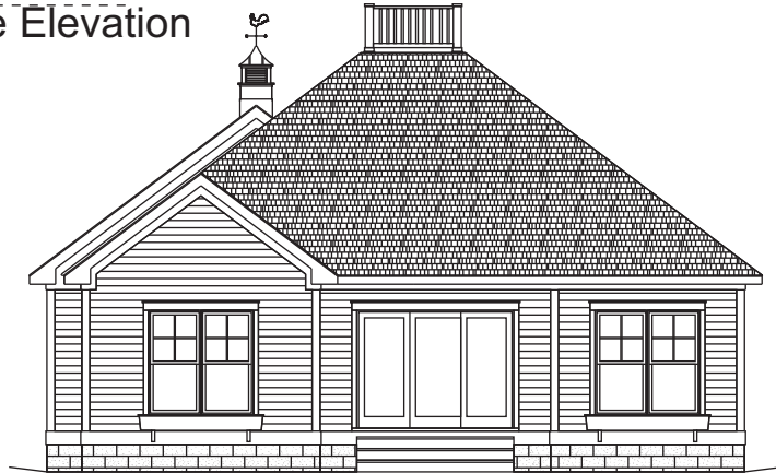
Street Side Elevation
