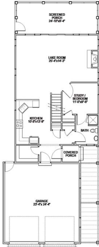
Main Level
